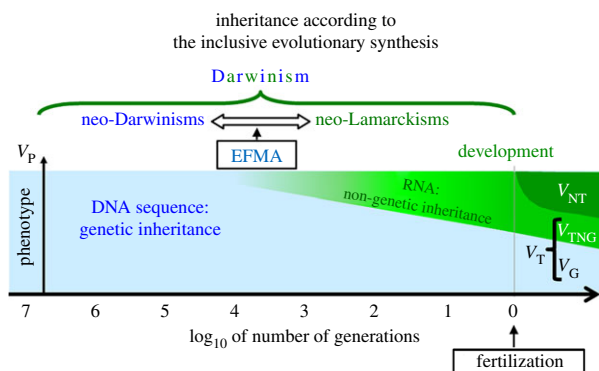
Figure 5. The concept of inheritance in the inclusive evolutionary synthesis. This synthesis unifies neo-Darwinism with neo-Lamarckism by rejuvenating Darwin's vision of inheritance. Blue hue (to the left) depicts the role of genetics, which constitutes the core idea of neo-Darwinism, stressing the major role of the DNA sequence. Green hue (to the right) represents components that are inherited non-genetically and are in part under environmental influence, which constitutes the main claim of (neo)-Lamarckism. RNAs constitute one of the major molecules of non-genetic inheritance of recently acquired characters. EFMA: Epigenetically-Facilitated Mutational Assimilation [19]. (Online version in colour.)
